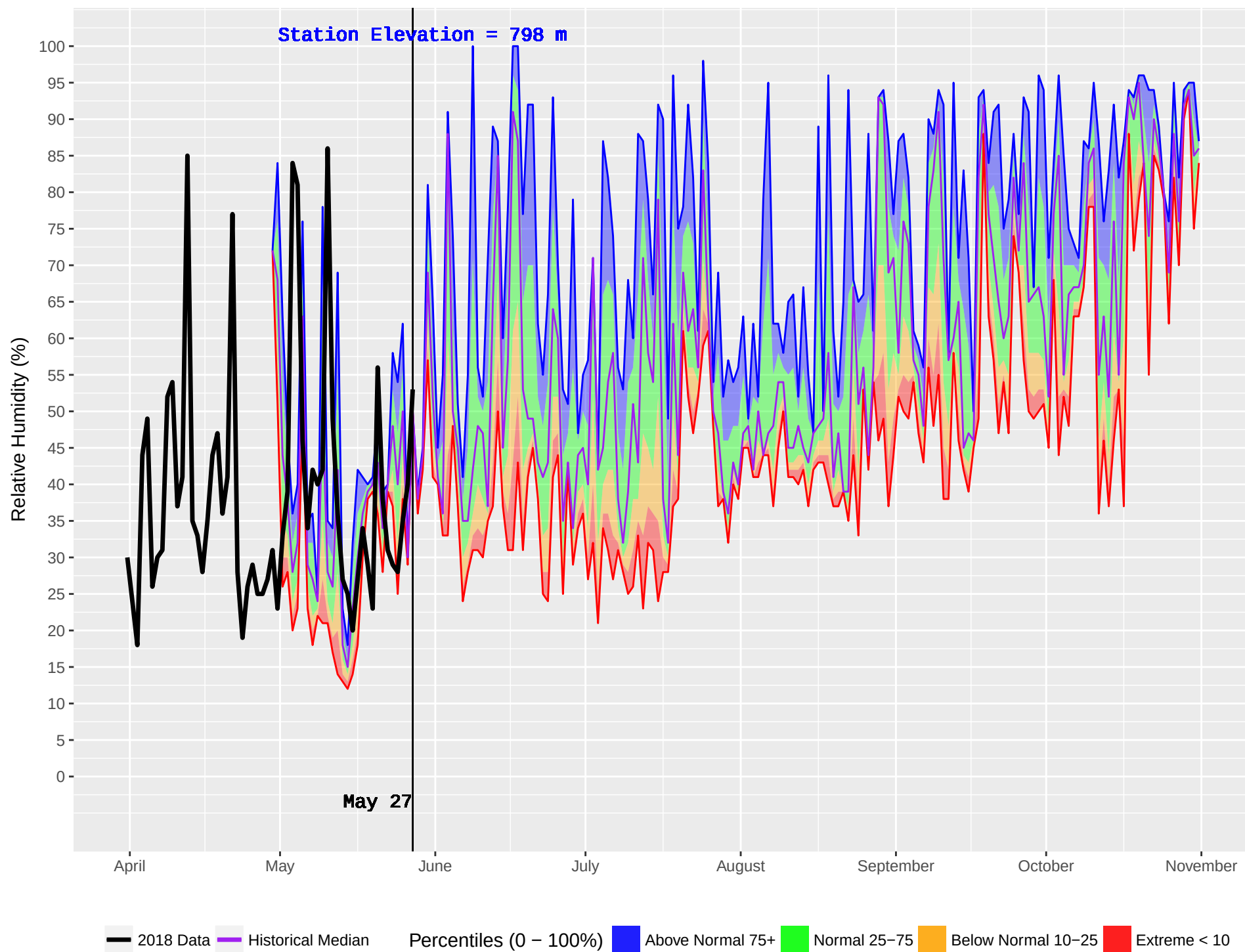
SEVEREID (1165) : Historical (2014–2016) and Current (2018) Noon Relative Humidity
