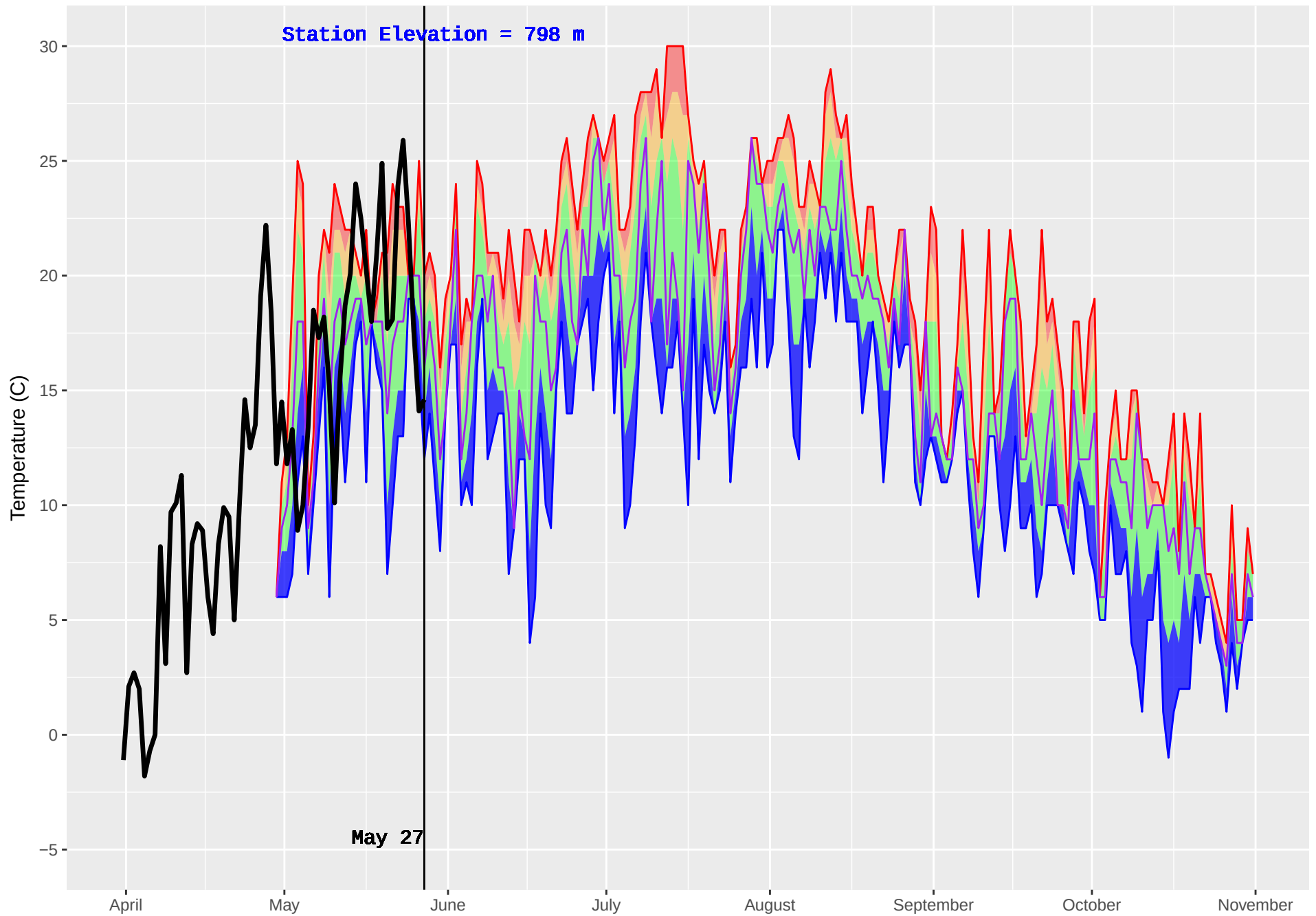
SEVEREID (1165) : Historical (2014–2016) and Current (2018) Noon Temperature
